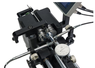
Anwendung Induktivtaster Example of use inductive probe
